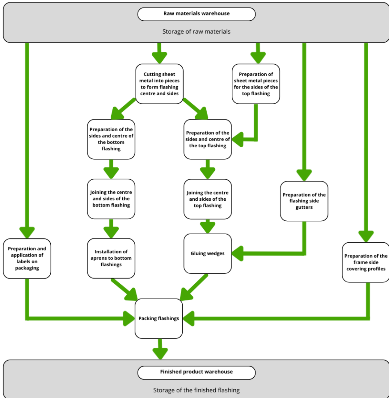
Figure 2. Production diagram of flashings for roof windows Standard manufactured by Fakro PP Sp. z o.o.
