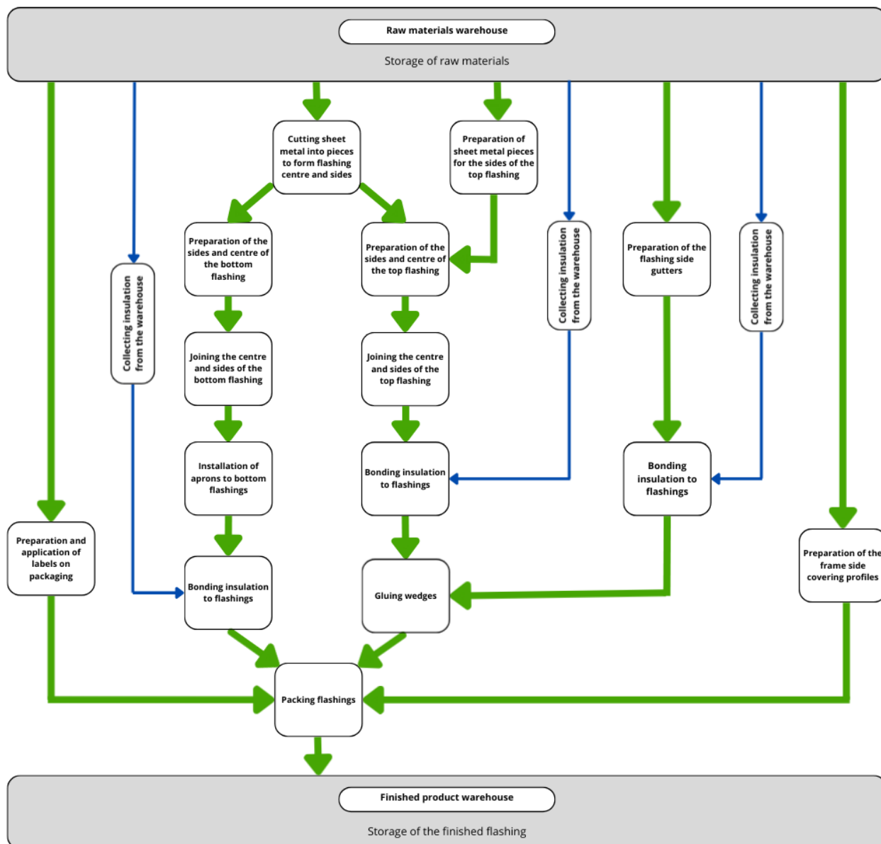
Figure 3. Production diagram of flashings for roof windows Thermo manufactured by Fakro PP Sp. z o.o.
