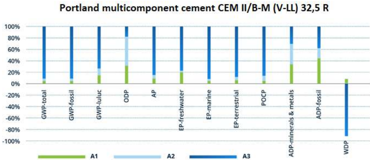
Figure 3. Shares of life cycle modules on the main categories of influence – portland multicomponent cement CEM II/B-M (V-LL) 32,5 R .
