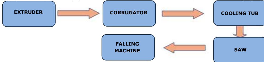
Figure 2: Process diagram of riser pipe PP DIAMIR in the production plant Kaczmarek-Malewo in Malewo.
